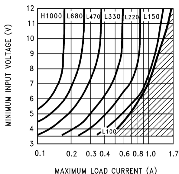
FIGURE 8. HS2577S/T_ADJ-15 Inductor Selection Guide
