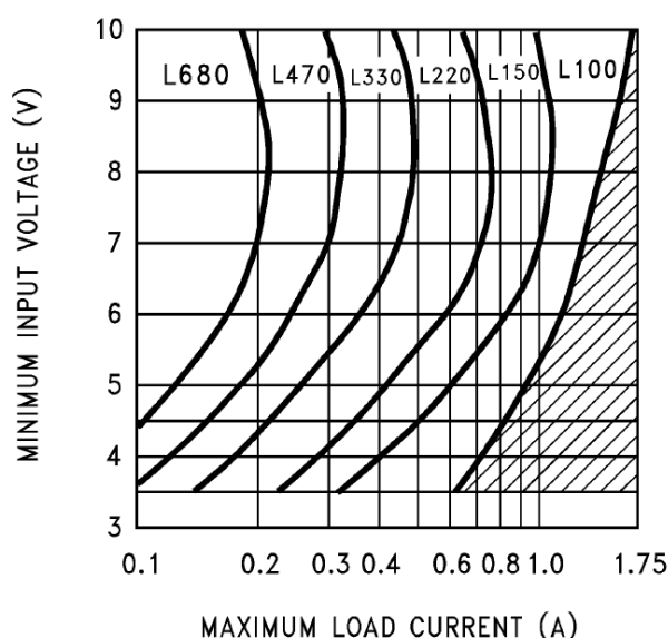
FIGURE 7. HS2577S/T_ADJ-12 Inductor Selection Guide
