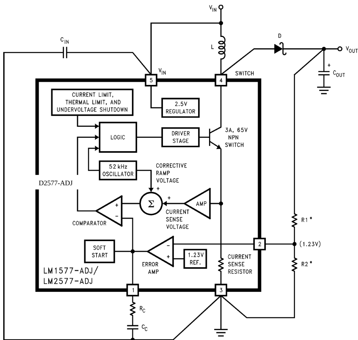
FIGURE 4. HS2577S/T_ADJ Block Diagram and Boost Regulator Application
