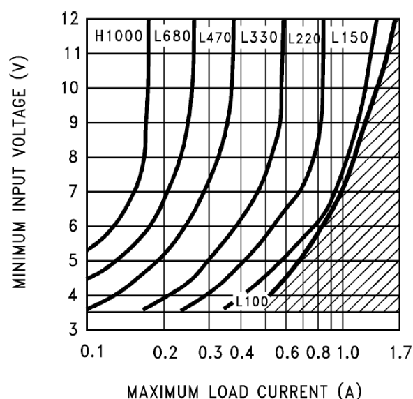
FIGURE 8. HS2585S/T_ADJ-15 Inductor Selection Guide
