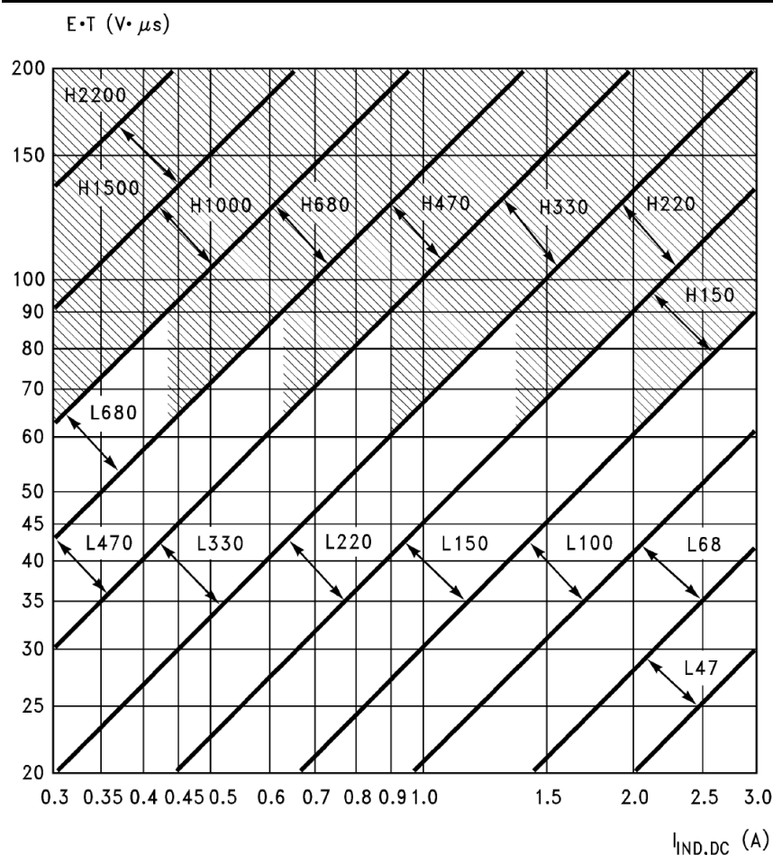
FIGURE 9. HS2585S/T_ADJ-ADJ Inductor Selection Graph
