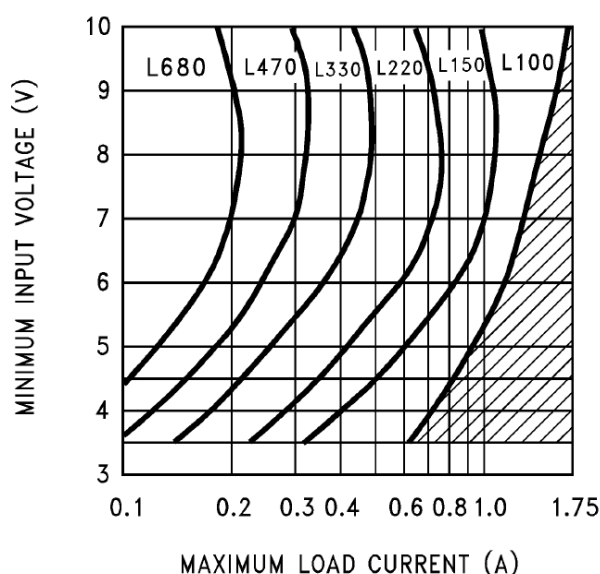
FIGURE 7. HS2585S/T_ADJ-12 Inductor Selection Guide
