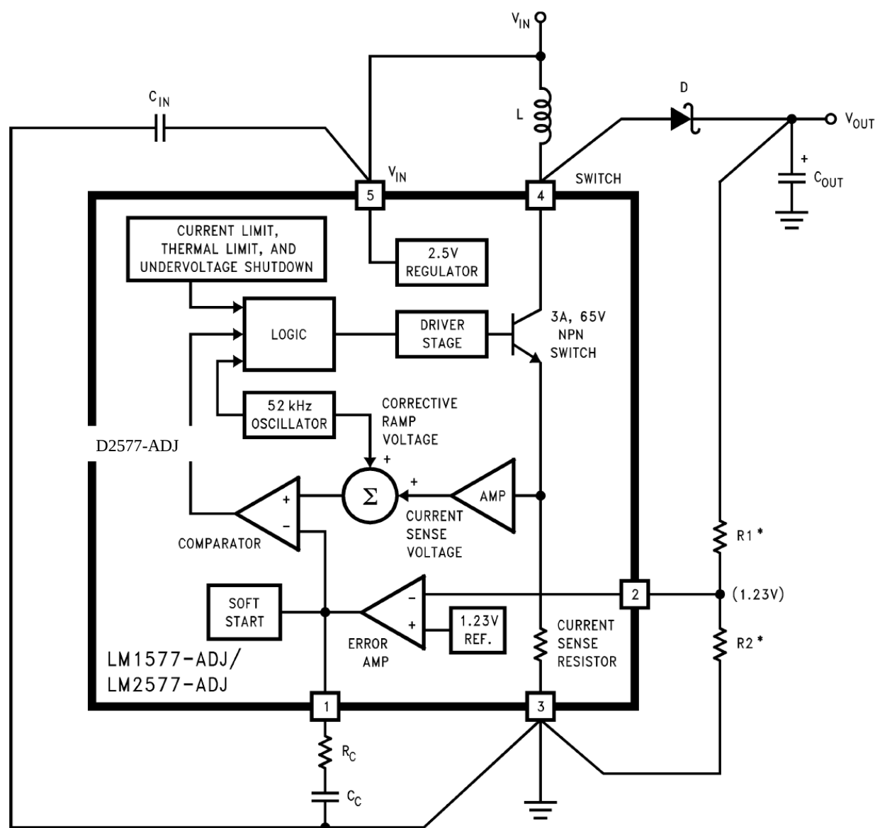
FIGURE 4. HS2585S/T_ADJ Block Diagram and Boost Regulator Application
