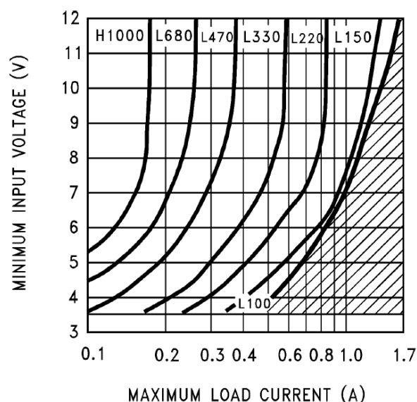
FIGURE 8. HS2587S/T_ADJ-15 Inductor Selection Guide
